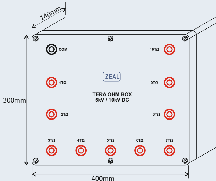
Fig. Isometric View
